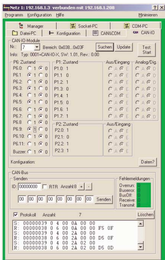
Abb. 15: Dialogbox CAN-IO
